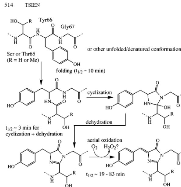
Figure 2 Mechanism proposed by Cubitt et al (22) for the intramolecular biosynthesis of the GFP chromophore, with rate constants estimated for the Ser65 → Thr mutant by Reid & Flynn (23) and Heim et al (25).
