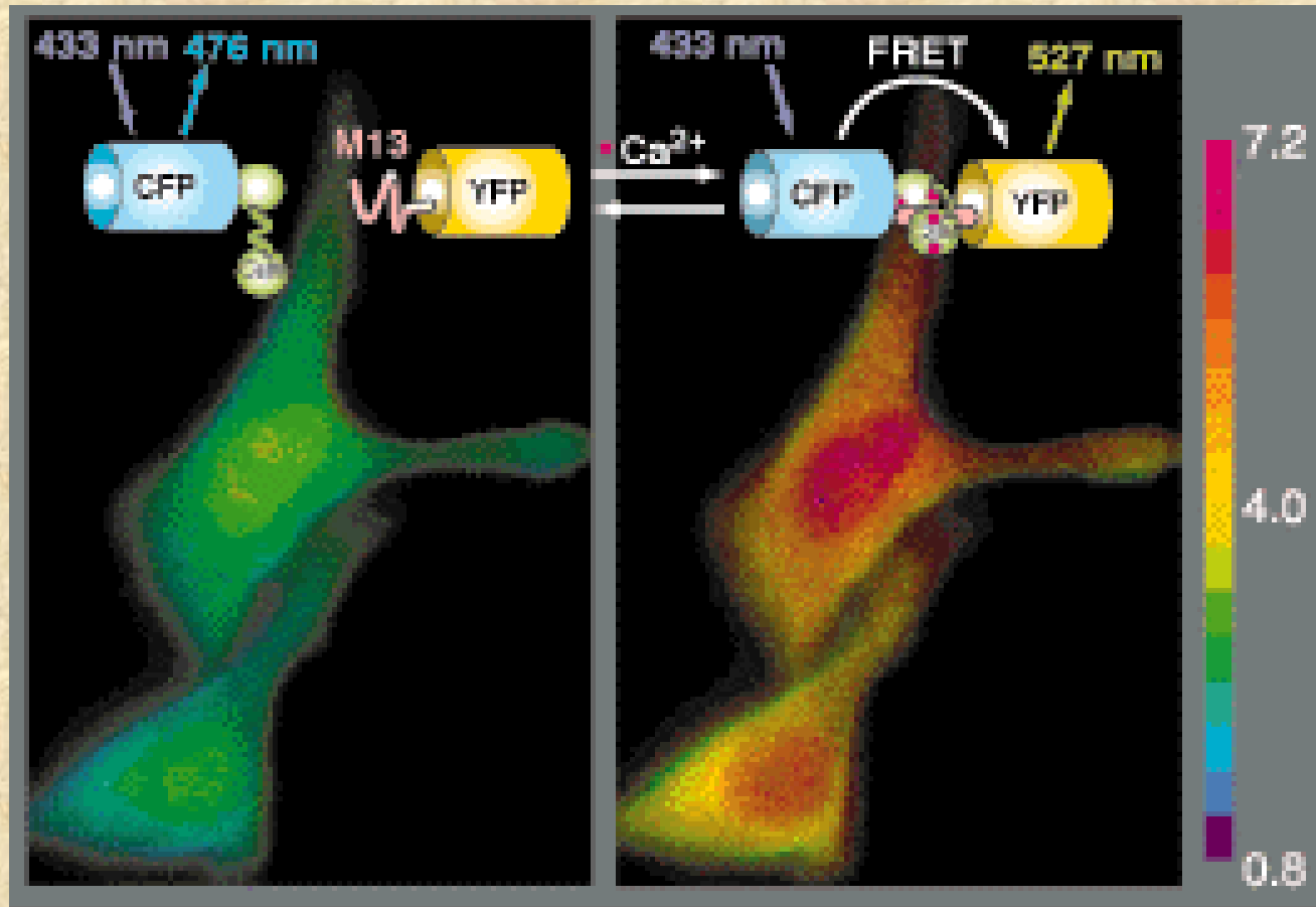
Fig. 1. Imaging by FRET of induced protein-protein interaction in individual live cells. Cyan-GFP-labeled calmodulin (CFP-CaM) and yellow-GFP-labeled calmodulin-binding peptide (M13-YFP) were coexpressed in HeLa cells (14). Pseudocolor hues from blue to magenta indicate increasing ratios of yellow to cyan emissions, resulting either from increased FRET (see overlaid schematic) or excess of YFP over CFP. The left panel shows two cells before stimulation, while the right panel shows the same cells after elevation of cytosolic \text{Ca}^{2+} by 0.1 mM histamine.
