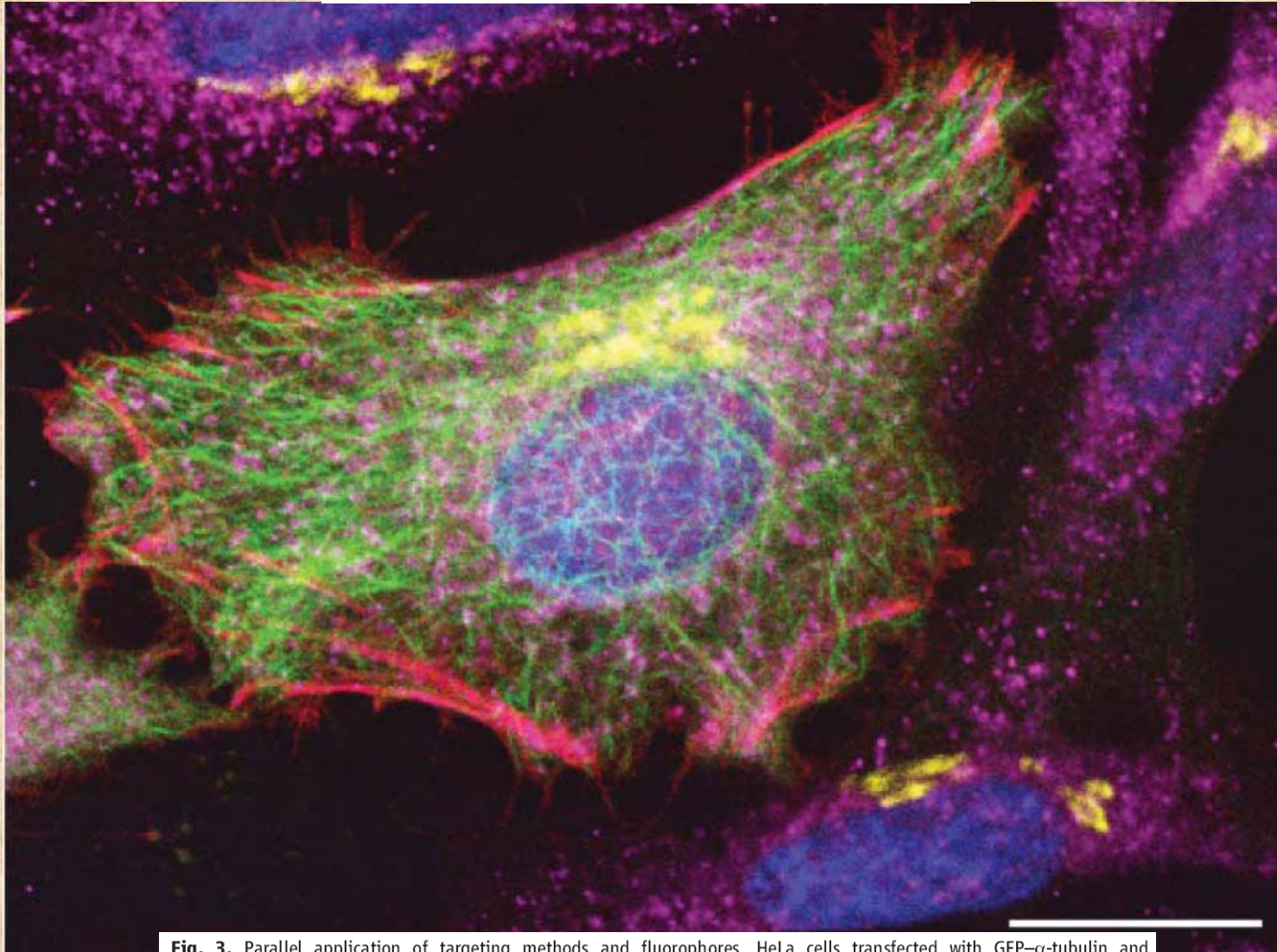
Fig. 3. Parallel application of targeting methods and fluorophores. HeLa cells transfected with GFP- \alpha -tubulin and tetracysteine- \beta -actin were stained with ReAsH. After fixation, cells were immunolabeled for the Golgi matrix protein giantin with QDs and for the mitochondrial enzyme cytochrome c with Cy5 as indicated. DNA was stained with Hoechst 33342. Images were acquired from Z planes that best represent each structure using excitation and emission wavelengths as indicated. Individual channels are false-colored (middle) and merged (bottom). Scale bars, 20 \mu m.
