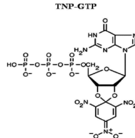
Figure 1. Structures of 4'-6-diamidino-2-phenylindole (DAPI) and 2',3'-O-(2,4,6-trinitrocyclohexadienylidene)-GTP (TNP-GTP) at neutral or basic pH.
