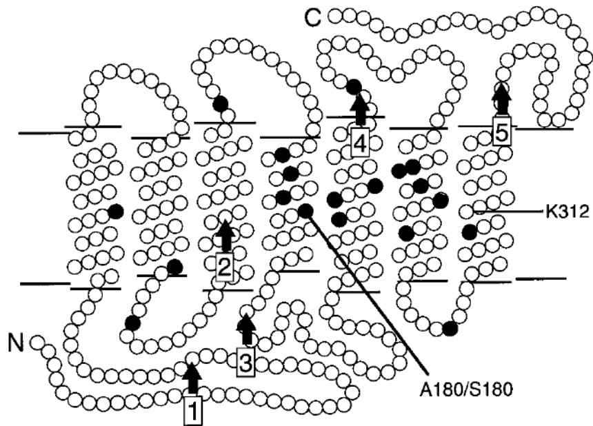
Figure 3. Schematic diagram of the human red and green pigments in the membrane. The N terminus ( N ) faces the extracellular space, and the C terminus ( C ) faces the cytosol. Each filled circle represents a position that differs between red and green pigments in the set of sequences studied here; these are positions 65, 111, 116, 153, 171, 174, 178, 180, 230, 233, 236, 249, 274, 275, 277, 279, 285, 298, and 309. The locations of lysine 312 ( K312 ), the site of covalent attachment of 11- cis retinal, and the polymorphic serine/alanine at position 180 ( A180/S180 ) are indicated. The five intron positions are indicated by vertical arrows.
